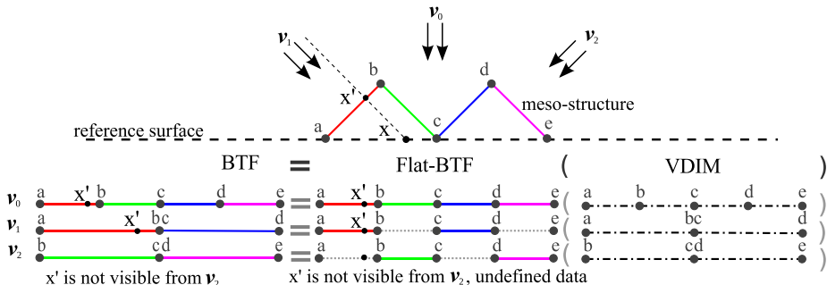
Figure 2: In a standard BTF, the appearance due to the meso-structure is computed or measured independently for a set of view directions \nu_0 , \nu_1 and \nu_2 . For each view, the visible illumination is stored but these data are deformed and stretched to fit the corresponding image space (for instance, segment ab is much longer in view \nu_1 than in view \nu_0 ). On the contrary, in our Flat-BTF model, the samples are stored according to their location on the meso-geometry. Then we use a view dependent indirection map (VDIM) to convert a Flat-BTF into standard BTF representation.
