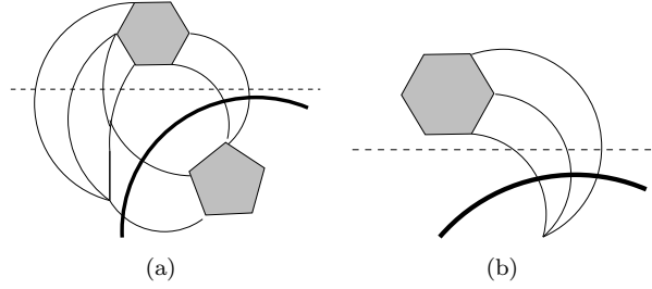
FIGURE 2. Conventions: 1.Filled polygons represent cliques, and curved arcs represent edges. 2.The dotted line separates C (the upper set of vertices) from Q . 3. The widest arc shows a minimal cut [S, \bar{S}] . Descriptions: (a) Here |[S, \bar{S}]| = k = 4 , \Phi = 4 , |\partial^1 Q| = 3 . (b) Here |[S, \bar{S}]| = k = 3 , \Phi = 1 , |\partial^1 Q| = 1 , Q = \partial^1 Q . This example shows that Corollary 2 includes an edge-connectivity version of the Expansion Lemma in [West, 2001], Lemma 4.2.3.
