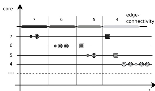
(b) Wide sense connectivity
