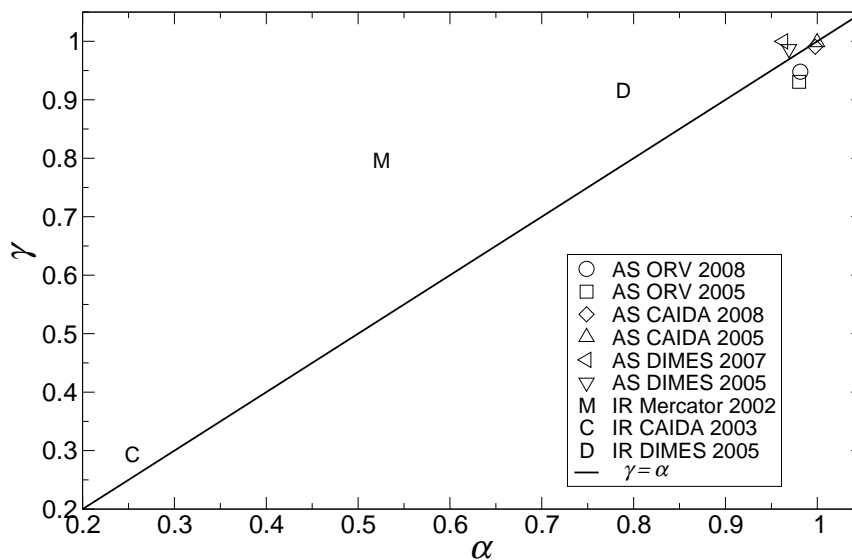
FIGURE 4. Comparison between \gamma and \alpha . The line \alpha = \gamma splits the space in two areas, the upper one for graphs with C concentrated on high populated shells ( \gamma > \alpha ), and the bottom for C mainly in low populated shells ( \gamma < \alpha ).
