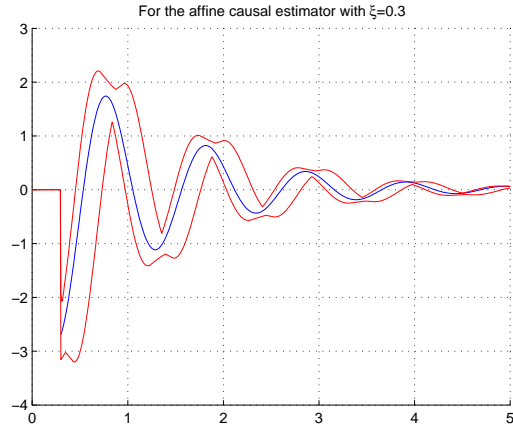
(a) e_{R_1}^-(k, \mu, -T, 2, \xi) and its bounds with \xi = 0.3
