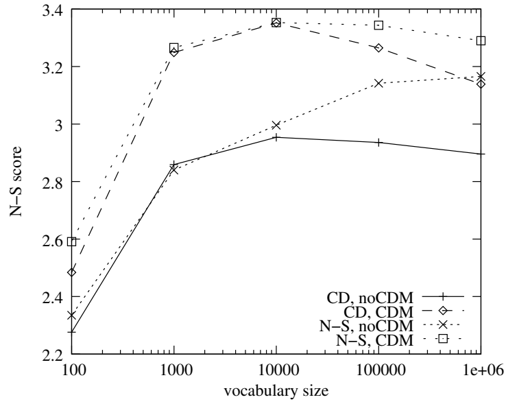
Figure 7: N-S dataset: impact of the vocabulary size and of the clustering dataset (independent dataset “CD” or the N-S set). These curves have been generated using the N-S preprocessed data [11]. Fixed parameter: n_N = 10 .
