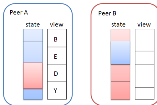
(c) Merge and update local state.
