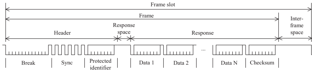
Figure 7: Format of the LIN frame. A frame is transmitted during its “frame slot” which corresponds to an entry of the schedule table
