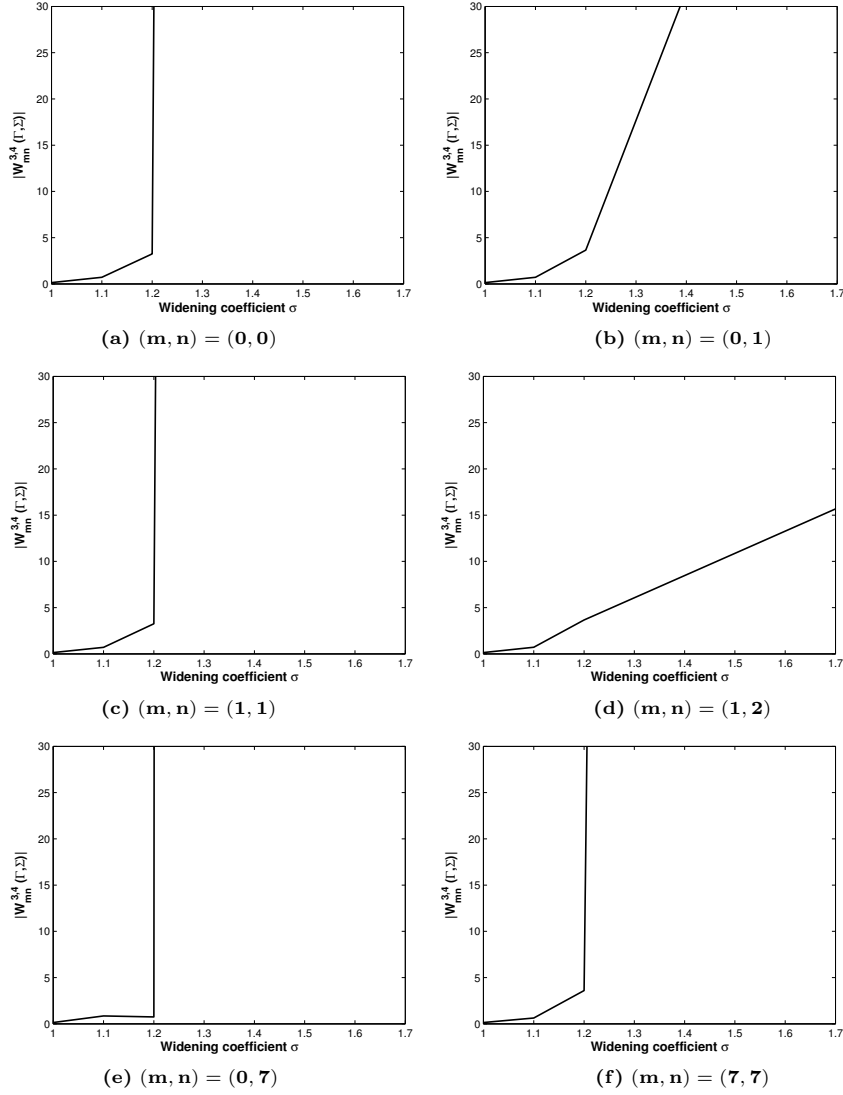
Figure 2: Sensitivity of the Wronskien-like function |W_{mn}^{3,4}(\Gamma, \Sigma)| given by Eq.(??) to the widening coefficient \sigma = \frac{a_\Sigma}{a_\Gamma} . Case where e_\Gamma = e_\Sigma = 0.9 and ka_\Gamma = 20 .
