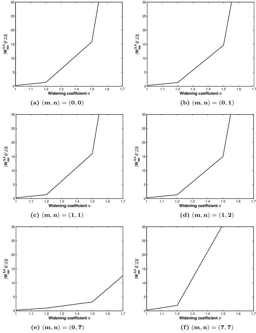
Figure 1: Sensitivity of the Wronskien-like function |W_{mn}^{3,4}(\Gamma, \Sigma)| given by Eq.(??) to the widening coefficient \sigma = \frac{a_\Sigma}{a_\Gamma} . Case where e_\Gamma = e_\Sigma = 0.9 and ka_\Gamma = 10 .
