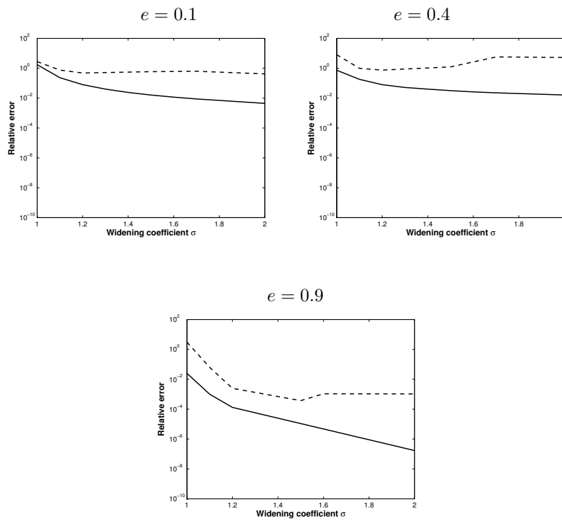
Figure 12: Sensitivity of the relative error to the widening parameter \sigma for ka = 20 and incident angle \varphi_0 = 0 ; DtN2 (plain), BGT2 (dashed).
