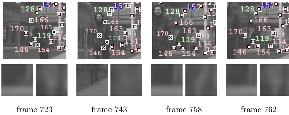
Fig. 13. Restarting the tracking of a temporary occluded group of features: tracked features and rejected projections are designated with squares and crosses, respectively. The bottom row shows the optimized warps for the features #146 (left) and #170 (right).
