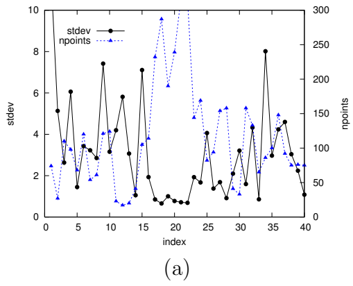
Fig. 9. Counts of mapped point features and reprojection errors plotted against the arcs of the two environment graphs. The data were obtained on the sequence ifsic5 , by employing approaches based on wide-baseline matching (a) and tracking (b) .
