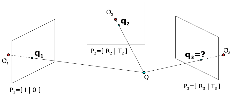
Fig. 5. The point transfer problem: given projections of some 3D point Q onto two images I_1 and I_2 , we wish to find its projection in a new view I_3 . The decomposed solution of that problem is: (i) image correspondences are used to recover the two-view geometry (I_1, I_2) ; (ii) the two projections \mathbf{q}_1 and \mathbf{q}_2 are used to triangulate the 3D point Q ; (iii) the two-view geometry (I_1, I_3) is recovered and put into the frame of the geometry (I_1, I_2) ; (iv) the desired point \mathbf{q}_3 is obtained by projecting Q onto camera 3.
