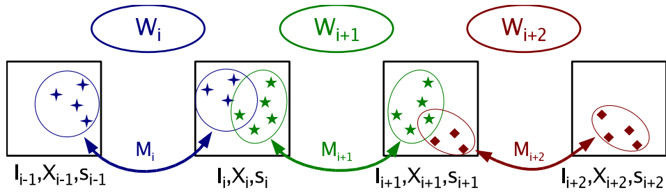
Fig. 3. The hybrid representation of a linear environment (the same indexing is used both for nodes and arcs): environment graph with key-images I_i , feature maps X_i , scale factors s_i and two-view geometries W_i . Match arrays M_i are also shown. See text for details.
