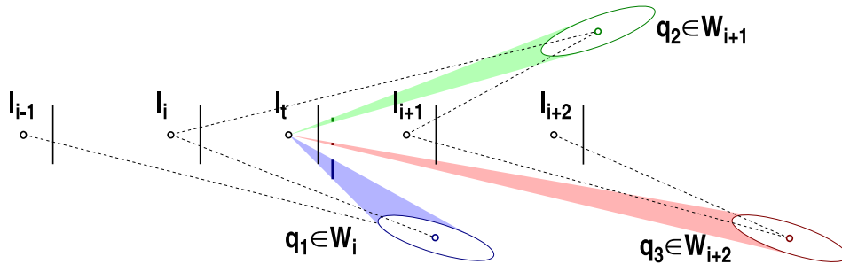
Fig. 6. Typical projections of the uncertainty ellipsoids for local reconstructions in the three arcs of the topological layer, for a prevalently forward movement.
