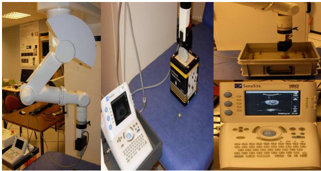
Fig. 7. Experimental setup: (left) medical robot equipped with an US probe transducer - (middle) interaction with an US phantom - (right) interaction with a lamb kidney immersed in a water-filled tank
