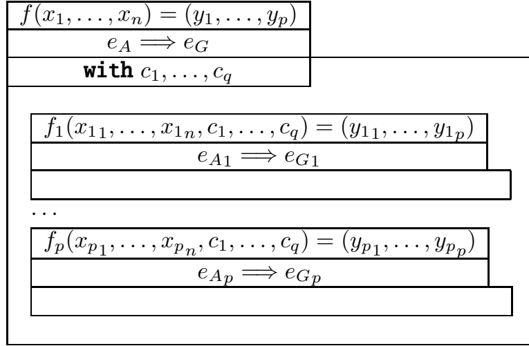
Figure 10: BZR composite node
