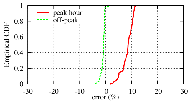
Figure 11: Empirical CDF of the error between the RTT measured at the source and estimated (Internet experiments).
