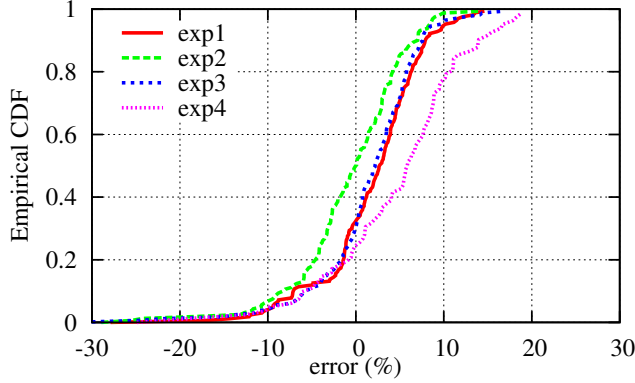
Figure 9: Empirical CDF of the error between the RTT measured at the source and the estimated RTT (testbed).
