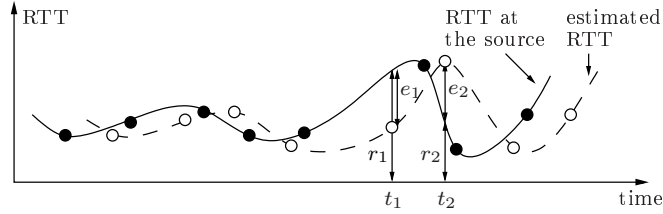
Figure 5: Errors in the RTT estimation process: a highly variable RTT induces bigger instantaneous estimation errors.
