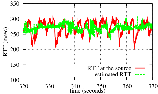
Figure 7: Example of the RTT measured at the source and the estimated RTT (exp2).
