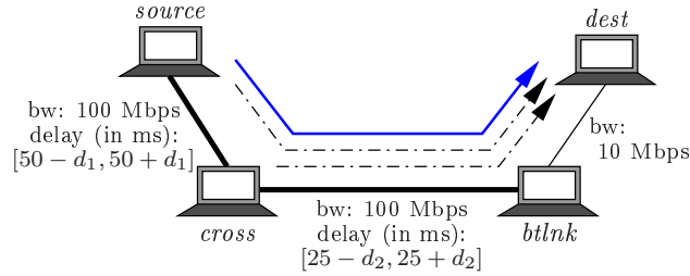
Figure 6: Scheme of the testbed: the continuous line represents the observed flow, dashed lines represent the cross traffic.
