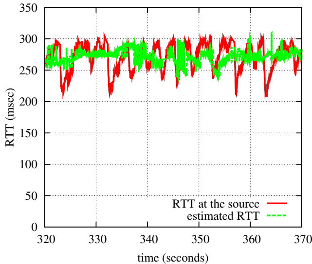
Figure 6: Example of the RTT measured at the source and the estimated RTT (exp2).
