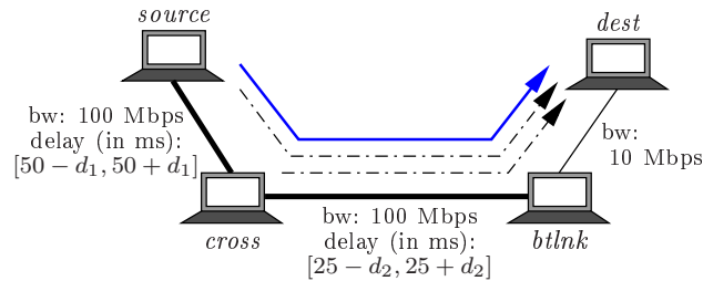
Figure 5: Scheme of the testbed: the continuous line represents the observed flow, dashed lines represent the cross traffic.
