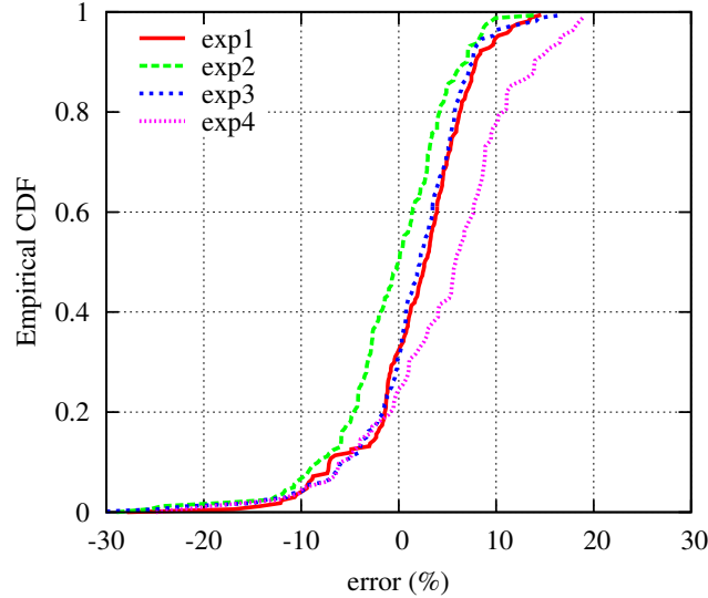
Figure 8: Empirical CDF of the error between the RTT measured at the source and the estimated RTT (testbed).
