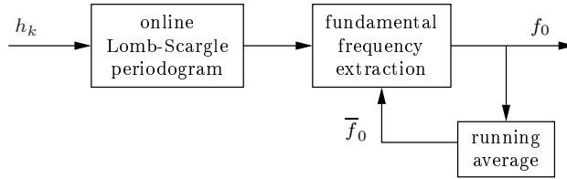
Figure 3: The RTT estimation process: after the update of the spectrum estimation, the fundamental frequency is extracted. The estimation of the RTT is the inverse of the fundamental frequency f_0 .
