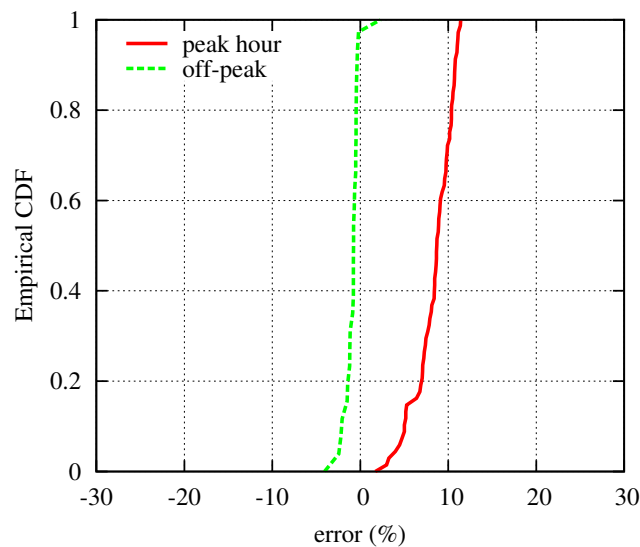
Figure 10: Empirical CDF of the error between the RTT measured at the source and estimated (Internet experiments).
