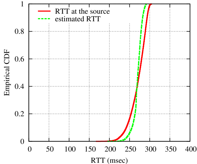
Figure 7: Empirical CDF of the RTT measured at the source and the estimated RTT (exp2).
