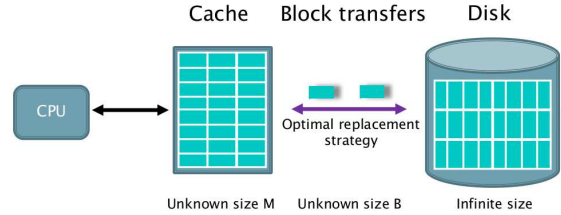
Figure 1: The cache-oblivious memory model
