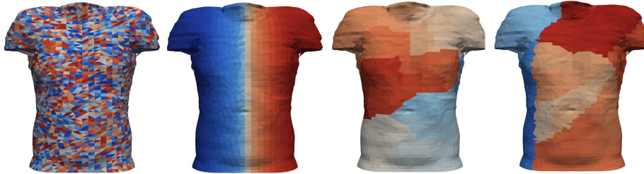
Figure 3: Visual illustration of different layouts for the torso mesh. Successive cells in memory are colored from blue to red. From left to right, the original, geometric (sorted by x, y and z coordinates), OpenCCL (cache-coherent layout from [26]) and FastCOL (our approach) layouts. For spatially close triangles, color discrepancy decreases from the left to right layouts. It denotes an improved memory locality, less likely to generate cache-misses for spatially coherent access patterns.
