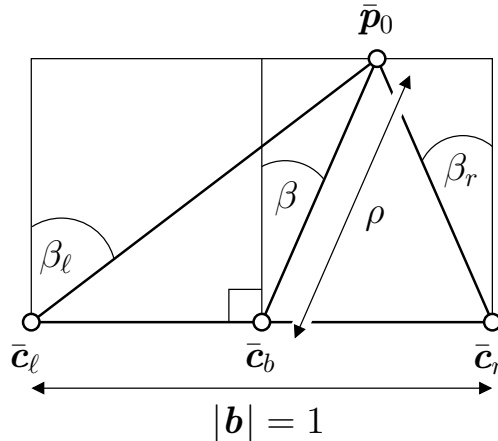
Figure 2: Binocular coordinates. The fixation point \bar{\mathbf{p}}_0 , in the visual plane \mathcal{V}_\alpha , is shown. The optical centres are indicated by \bar{\mathbf{c}}_\ell and \bar{\mathbf{c}}_r . The azimuth angles \beta and \beta_\ell are positive in this example, whereas \beta_r is negative. The cyclopean range of the fixation point is \rho .
