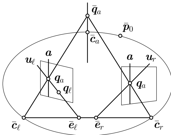
Figure 5: Construction of the epipolar geometry. Point q_\ell is given, so the epipolar line in \mathcal{I}_\ell is \mathbf{u}_\ell = \mathbf{q}_\ell \times \mathbf{e}_\ell . This line intersects the image \mathbf{a} of the midline horopter in \mathcal{I}_\ell at \mathbf{q}_a = \mathbf{a} \times \mathbf{u}_\ell . The point \mathbf{q}_a is on \mathbf{a} , and is therefore fixed, having the same coordinates \mathbf{q}_a in \mathcal{I}_r . It follows that the epipolar line in \mathcal{I}_r is \mathbf{u}_r = \mathbf{e}_r \times \mathbf{q}_a . The location of \mathbf{q}_r , which corresponds to \mathbf{q}_\ell , is unknown, but it must lie on \mathbf{u}_r . The Vieth-Müller circle, determined by the fixation point \bar{\mathbf{p}}_0 , is shown in the figure, as is the midline-horopter, which passes through points \bar{\mathbf{c}}_a and \bar{\mathbf{q}}_a .
