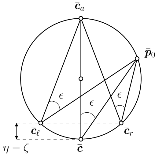
Figure 4: Version geometry. The points \bar{c}_a and \bar{p}_0 inscribe the version angle, \epsilon , at an optical centre, \bar{c} , which is located on the backward ( z < 0 ) arc of the Vieth-Müller circle. The same angle is inscribed at \bar{c}_\ell and \bar{c}_r . It follows that as \bar{p}_0 is fixated, \bar{c}_a lies in the same visual direction from each eye. Furthermore, the triangle defined by \bar{c}_\ell , \bar{c}_r , and \bar{c}_a is isosceles, and so the point \bar{c}_a is at the same distance from each eye.
