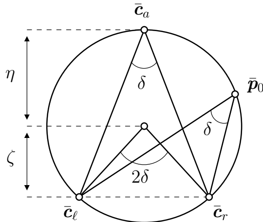
Figure 3: Vergence geometry. The Vieth-Müller circle is defined by the positions of the optical centres \bar{c}_\ell and \bar{c}_r , together with the fixation point, \bar{p}_0 . The forward ( z > 0 ) arc of the circle intersects the mid-sagittal plane at the point \bar{c}_a . The vergence angle, \delta , is inscribed at \bar{p}_0 by \bar{c}_\ell and \bar{c}_r . The same angle is inscribed at all other points on the circle, including \bar{c}_a .
