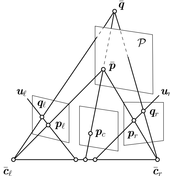
Figure 6: Geometry of cyclopean parallax. The fixation plane \mathcal{P} is defined by the fixation point, and is parallel to the cyclopean image plane. Any point \mathbf{p}_c defines a cyclopean ray, which intersects the fixation plane at \bar{\mathbf{p}} , and the scene at \bar{\mathbf{q}} . The scene point \bar{\mathbf{q}} has depth s with respect to \mathcal{P} . The predicted image-projections of \bar{\mathbf{q}} are at \mathbf{p}_\ell and \mathbf{p}_r . The true projections, \mathbf{q}_\ell and \mathbf{q}_r , are displaced along the corresponding epipolar lines, \mathbf{u}_\ell and \mathbf{u}_r , respectively. The displacement can be parameterized by s , as described in the text.
