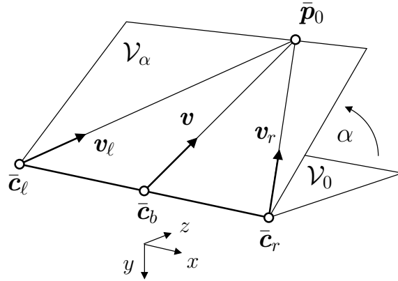
Figure 1: Visual directions. A visual plane \mathcal{V}_\alpha is defined by the optical centres \bar{\mathbf{c}}_\ell and \bar{\mathbf{c}}_r , together with the fixation point \bar{\mathbf{p}}_0 . The visual directions \mathbf{v} , \mathbf{v}_\ell and \mathbf{v}_r lie in this plane, which has an elevation angle \alpha . The scene coordinates are located at the cyclopean point \bar{\mathbf{c}}_b = (0, 0, 0)^\top , such that \mathcal{V}_0 coincides with the x, z plane.
