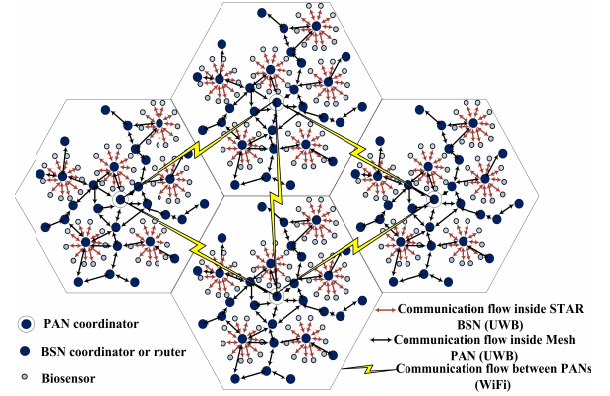
Fig. 4. WHSN architecture
