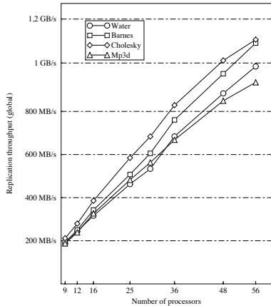
Figure 9: Recovery data throughput when varying the number of processors
