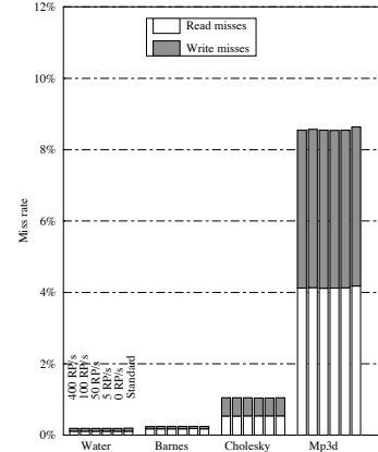
Figure 5: Node miss rate when varying the recovery point frequency
