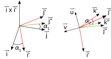
Figure 5: Rotation ( \vec{R}_1, \alpha_1 ) and rotation ( \vec{i}', \alpha_2 ).
