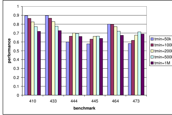
Figure 9: Normalized performance for Lag-0 WU-1 and various values of t_{min} on a subset of the benchmarks when T_{amb} = 50^\circ\text{C} .
