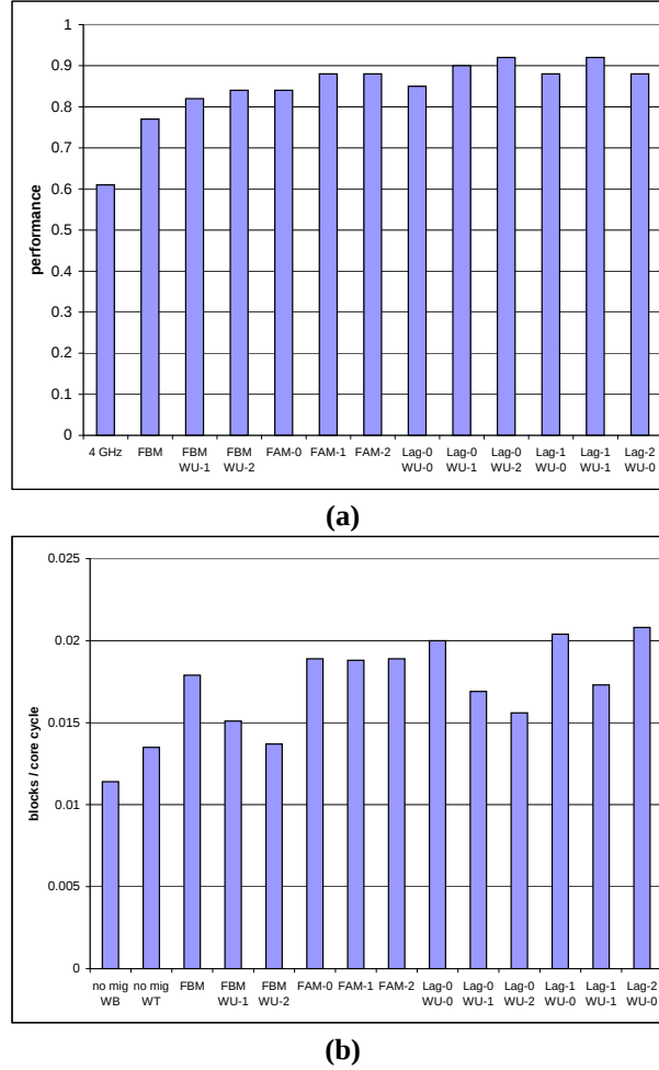
Figure 5: Graph (a) shows the performance of the different schemes when the migration interval is fixed to 200,000 cycles (8 GHz). Performance is normalized to the baseline (8 GHz, no migration). For each scheme, the bar represents the harmonic mean of the normalized performance over all benchmarks. Graph (b) shows the shared-bus activity, in blocks per core cycle. For each scheme, the bar represents the arithmetic mean over all benchmarks. The two leftmost bars are for the baseline with migration disabled, with a write-back and write-through L2 respectively.
