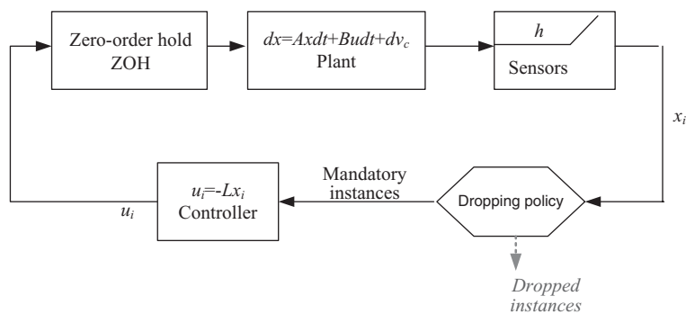
Figure 5.2. Control system architecture.
