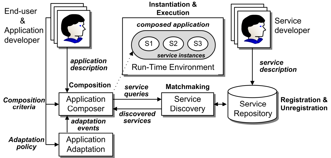
Fig. 1. Generic application composition process.
