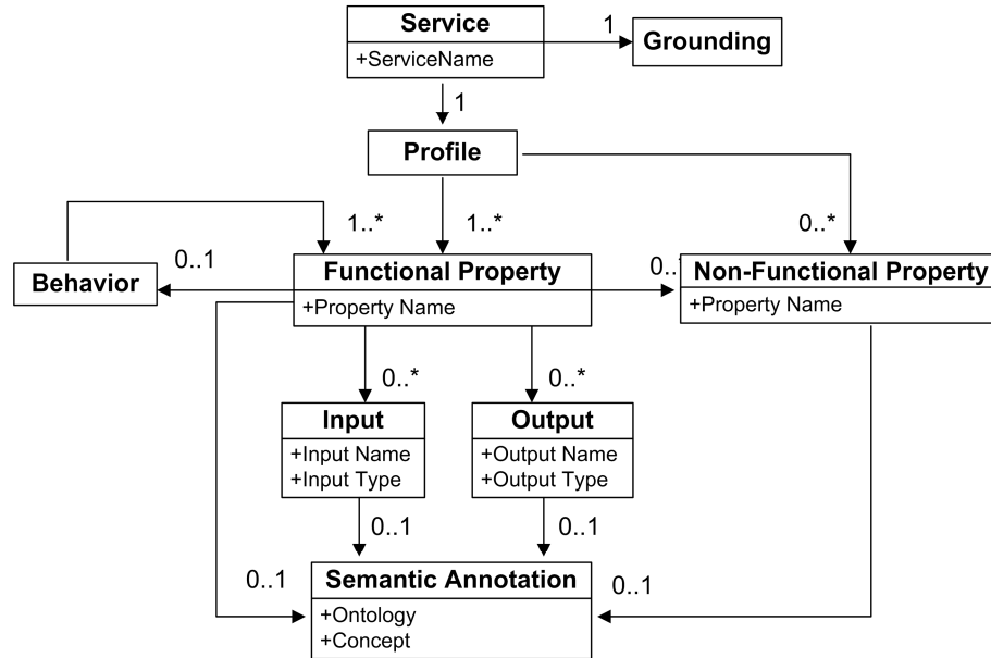
Fig. 9. Amli Service Description Model (AMSD), adapted from Ben Mokhtar (2007).
