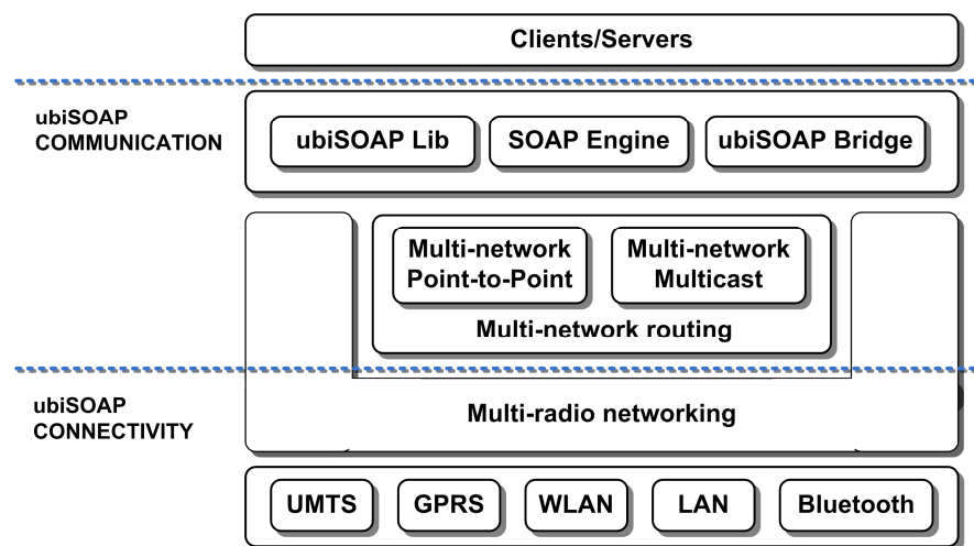
Fig. 8. ubiSOAP architecture. Adapted from Caporuscio et al (2009).
