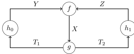
Figure 1: A simple example of Kahn network
