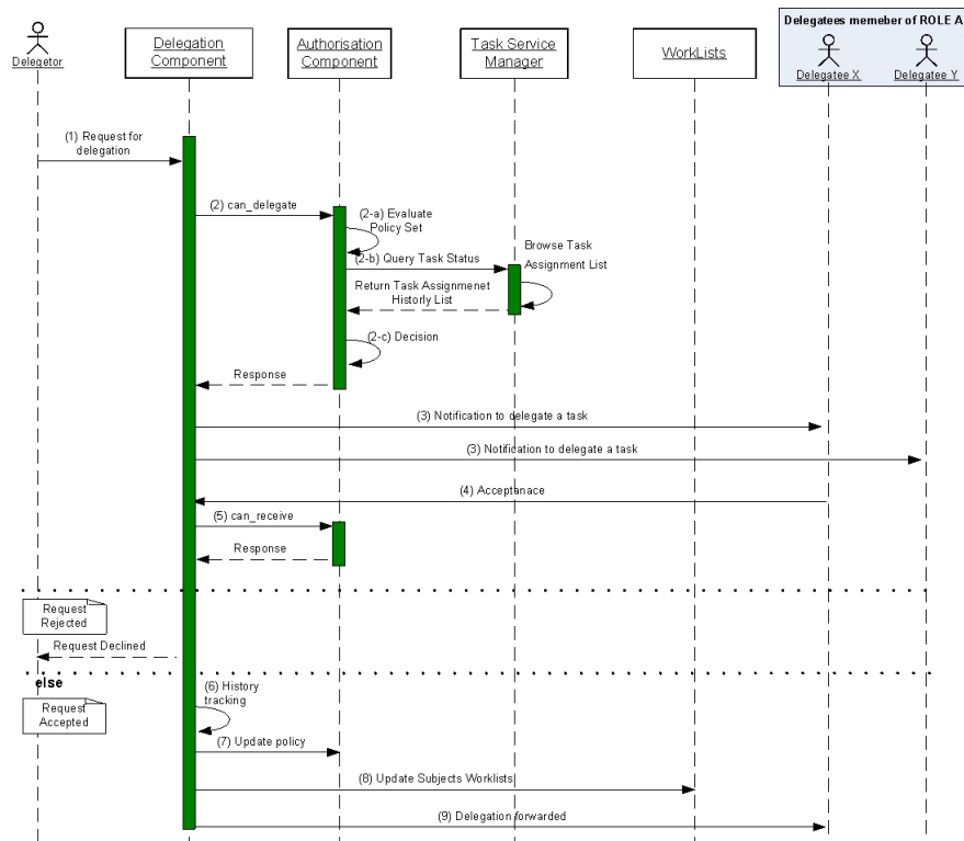
Figure 5. Task delegation protocol
