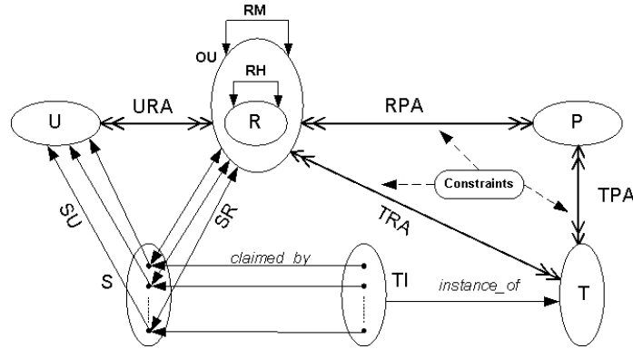
Figure 4. Task-oriented access control model
