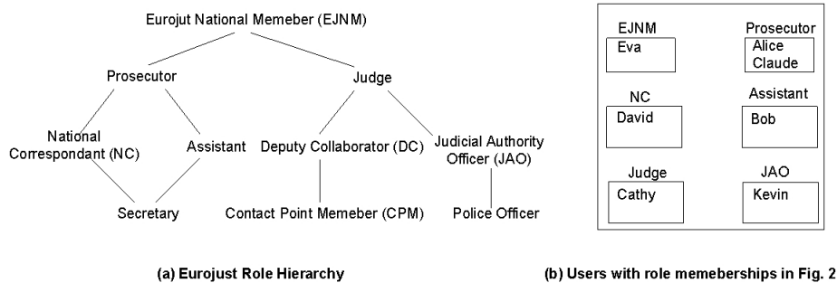
Figure 1. An example of organisational role hierarchy and users in Eurojust
