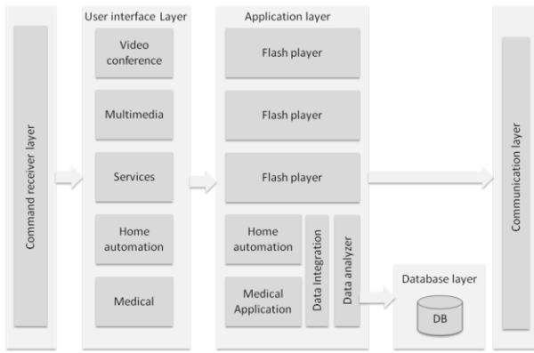
Fig. 3. Software architecture
