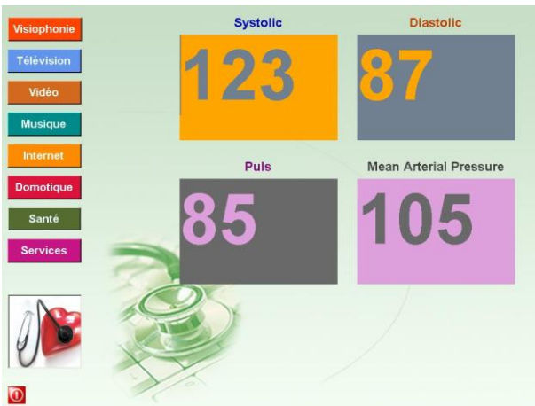
Fig. 4. Medical Interface
