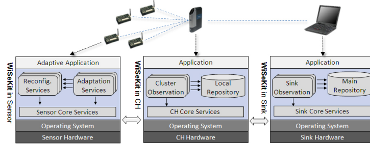
Fig. 2. WiSeKit in the hierarchical WSN architecture.
