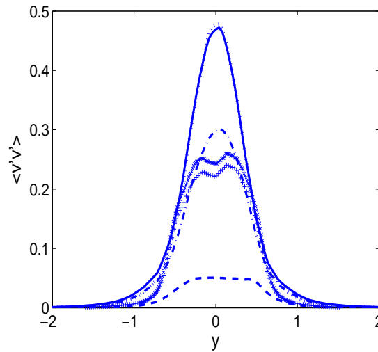
Figure 16: Total resolved streamwise Reynolds stress \langle v'v' \rangle at x = 1.54 , experiments: Parnaudeau et al.; --: Simu1; -: Simu2;...: Simu3; -.: Simu4; +: PIV1 experiment; \times : PIV2 experiment
