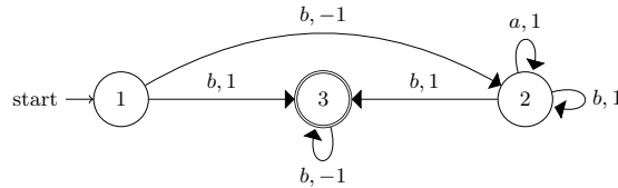
Fig. 2. \max/+ -automata \mathcal{A}_{exe3}
