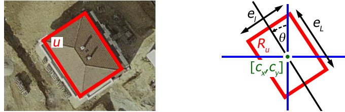
Figure 3: Description of the rectangle parameters
