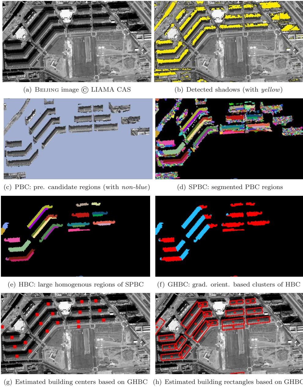
Figure 11: Illustration of the homogeneity based pre-detection
