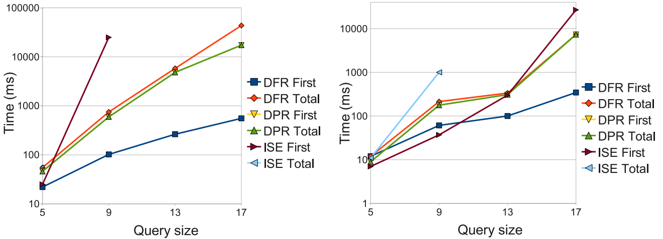
Figure 11: Query rewriting times.
