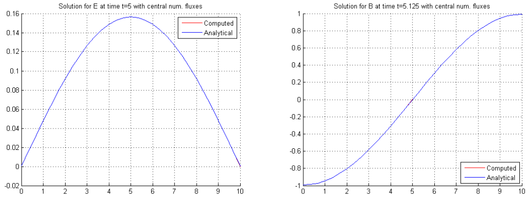
Fig. 11: Solution of Maxwell's equations using the DG method with central numerical fluxes and the time step such that stability condition is surely fulfilled (numerical solution totally fits analytical)
