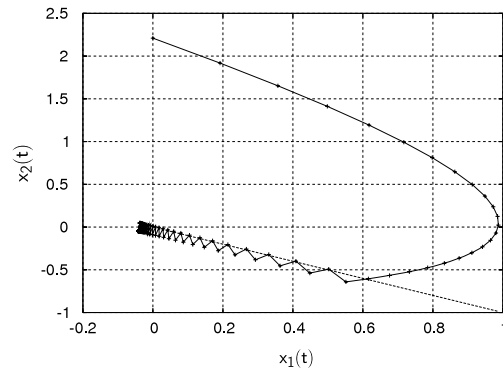
(b) h = 0.1 . Explicit Euler.
