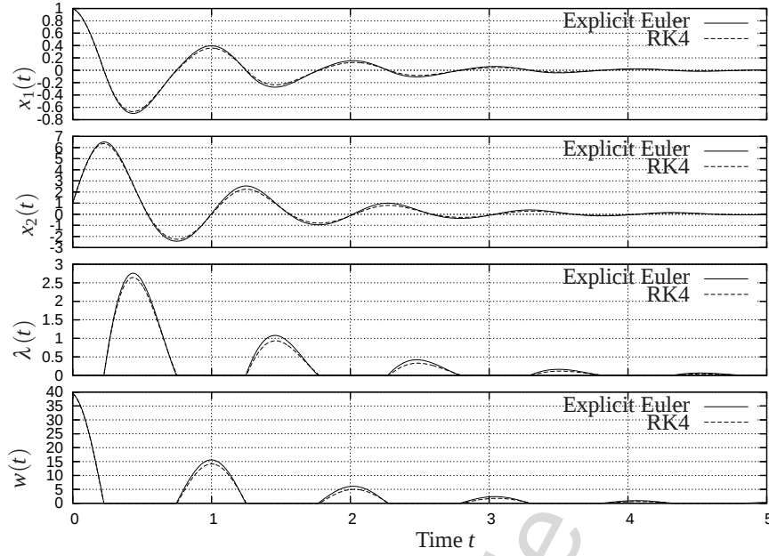
Fig. 1.5. Simulation of the circuit (b) with the initial conditions x_1(0) = 1 , x_2(0) = 1 and R = 10 , L = 1 , C = \frac{1}{(2\pi)^2} . Time step h = 5 \times 10^{-3}
