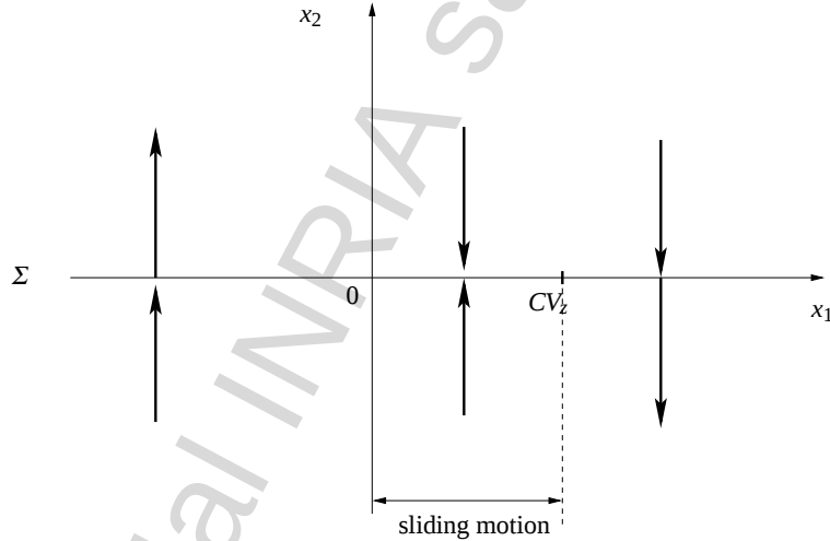
Fig. 1.10. The vector field on the switching surface \Sigma
