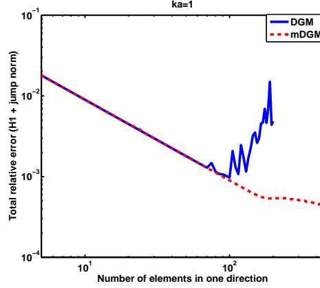
Figure 5: Convergence rates R-4-2 element
