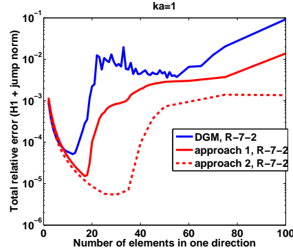
Figure 12: Convergence rates for the R-7-2 element
