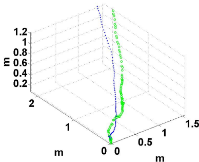
Figure 7: Results from the EKF which estimates the entire non-observable state. The 3 D trajectory is displayed. The blue dots indicate the ground truth while the green circles the estimated trajectory.
