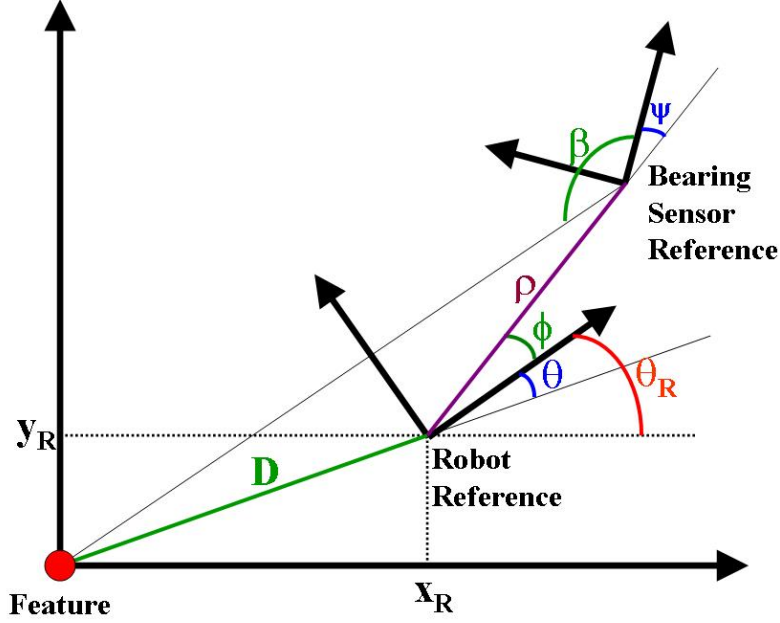
Figure 3: The two reference frames respectively attached to the robot and to the bearing sensor.
