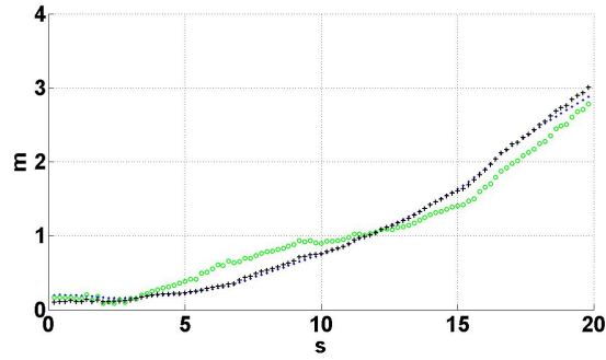
Figure 8: The true distances (blue dots), the value of the distances obtained from the values of x, y and z shown in figure 7 (green circles) and the distances estimated by implementing an EKF which directly estimates the observable modes (black crosses).
