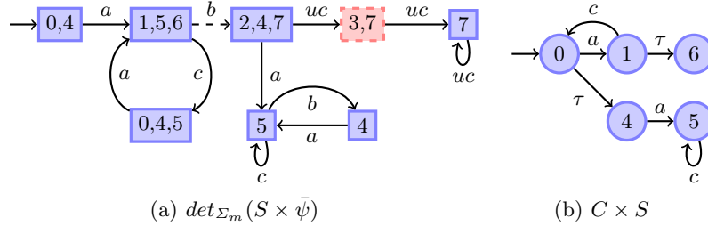
Fig. 3. Ensuring an integrity property by control
