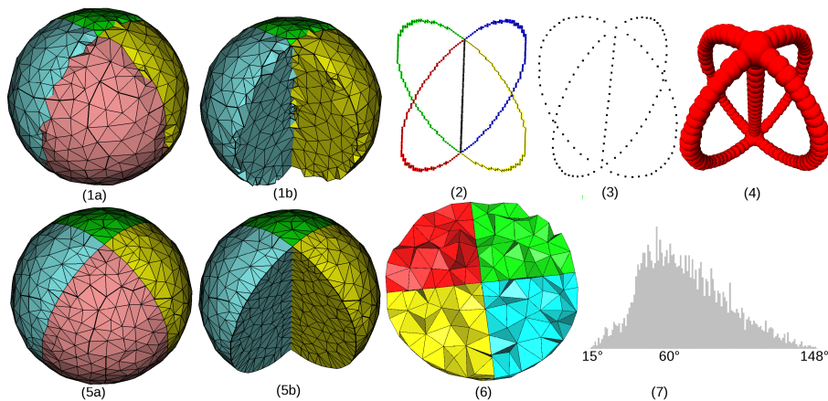
Fig. 2. (1) Delaunay refinement 3D mesh. (2) Multimaterial junctions: five 1-junctions and two 0-junctions. (3) Sampled points on junctions. (4) Protecting balls. (5) Edge preserving Delaunay refinement 3D mesh. (6) A cut of the tetrahedral mesh. (7) Dihedral angles distribution.
