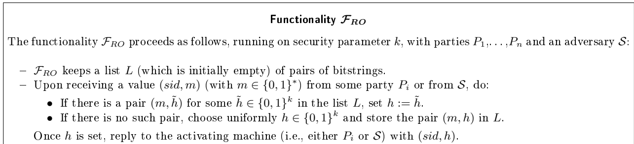
Fig. 4. Functionality \mathcal{F}_{RO}
