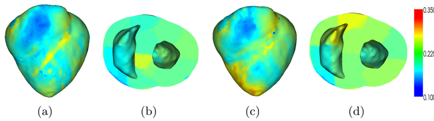
Fig. 6. Estimated Parameter \zeta_{close} comparison after personalisation with pacing location LV-Endo (a) (b), and RV-Epi (c) (d) (Epicardial and Myocardial (SA) views).
