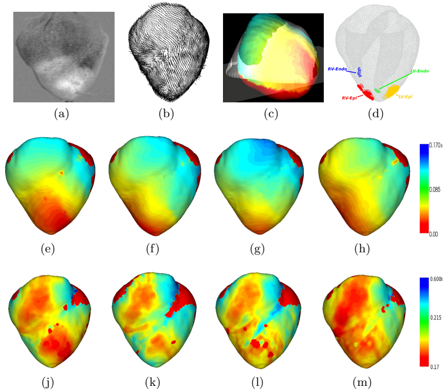
Fig. 2. (a) Optical Data, (b) Volumetric myocardial mesh generated from DT-MRI data with fibres, (c) Projection of depolarisation time isochrones (in s) derived from the filtered optical data to Volumetric Myocardial Mesh, (d) 4 pacing locations for LV-Epi, RV-Epi, LV-Endo and RV-Endo, (e) - (h) epicardial depolarisation isochrones and (j) - (m) repolarisation isochrones for LV-Epi, RV-Epi, LV-Endo, RV-Endo successively.
