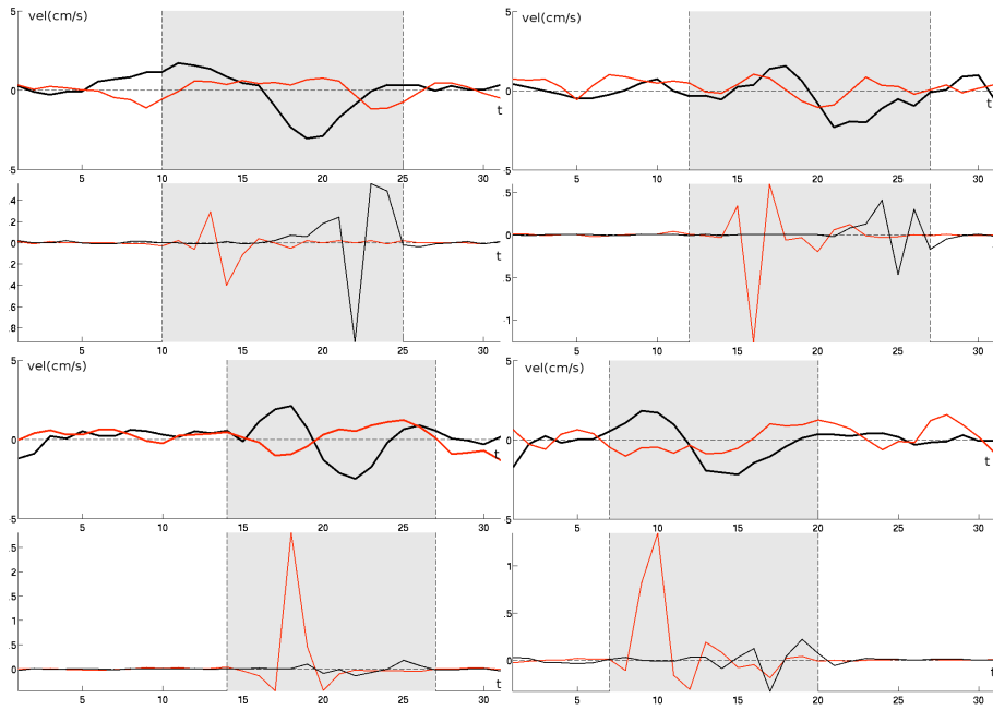
Fig. 2. Velocity profiles (top in each subplot) corresponding to pre- (black) and post-CRT (red) data, together with EGMs (bottom in each subplot) of EP_{elat} and EP_{lat} (black and red, respectively) for cases with septal flash. The dashed markers and grey area define the septal flash interval.
