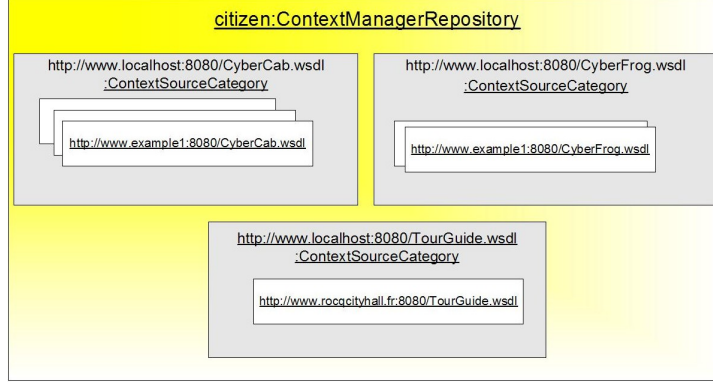
(a) Repository structure.
