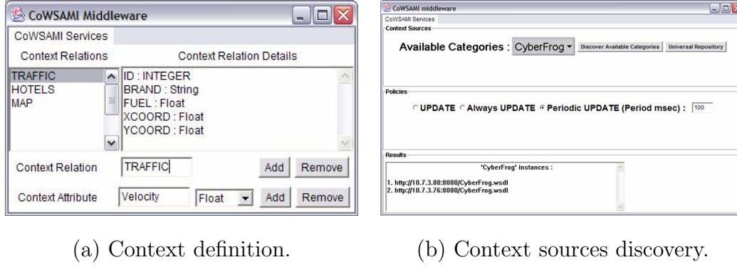
Fig. 12. CoWSAMI user interfaces.
