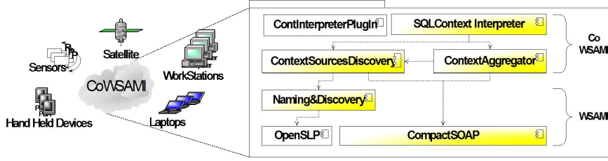
Fig. 2. CoWSAMI Architecture.
