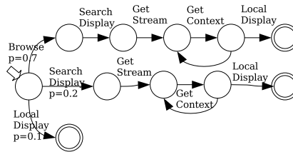
Fig. 8. Automaton of the e-movie application
