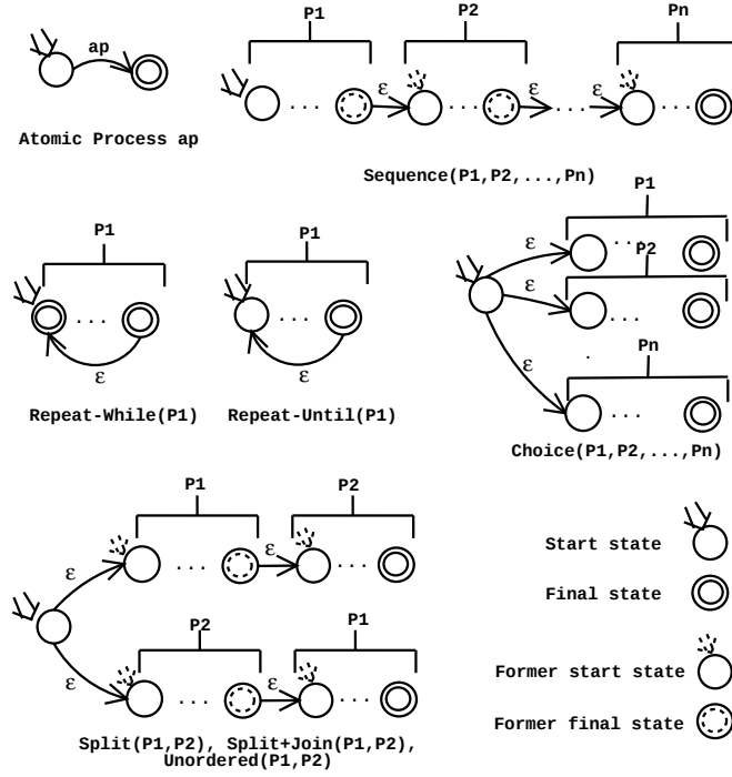
Fig. 7. Modeling OWL-S processes as finite state automata
