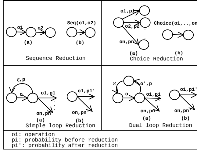
Fig. 9. Workflow Constructs
