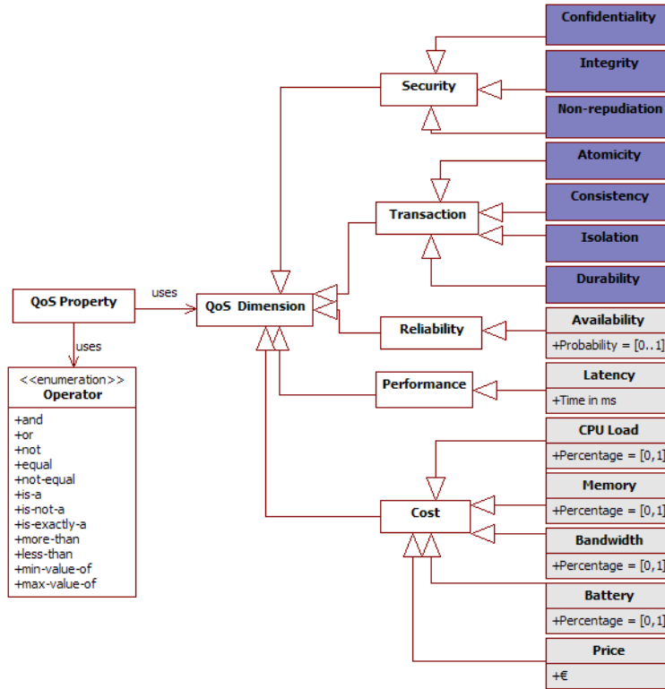
Fig. 6. QoS Specification
