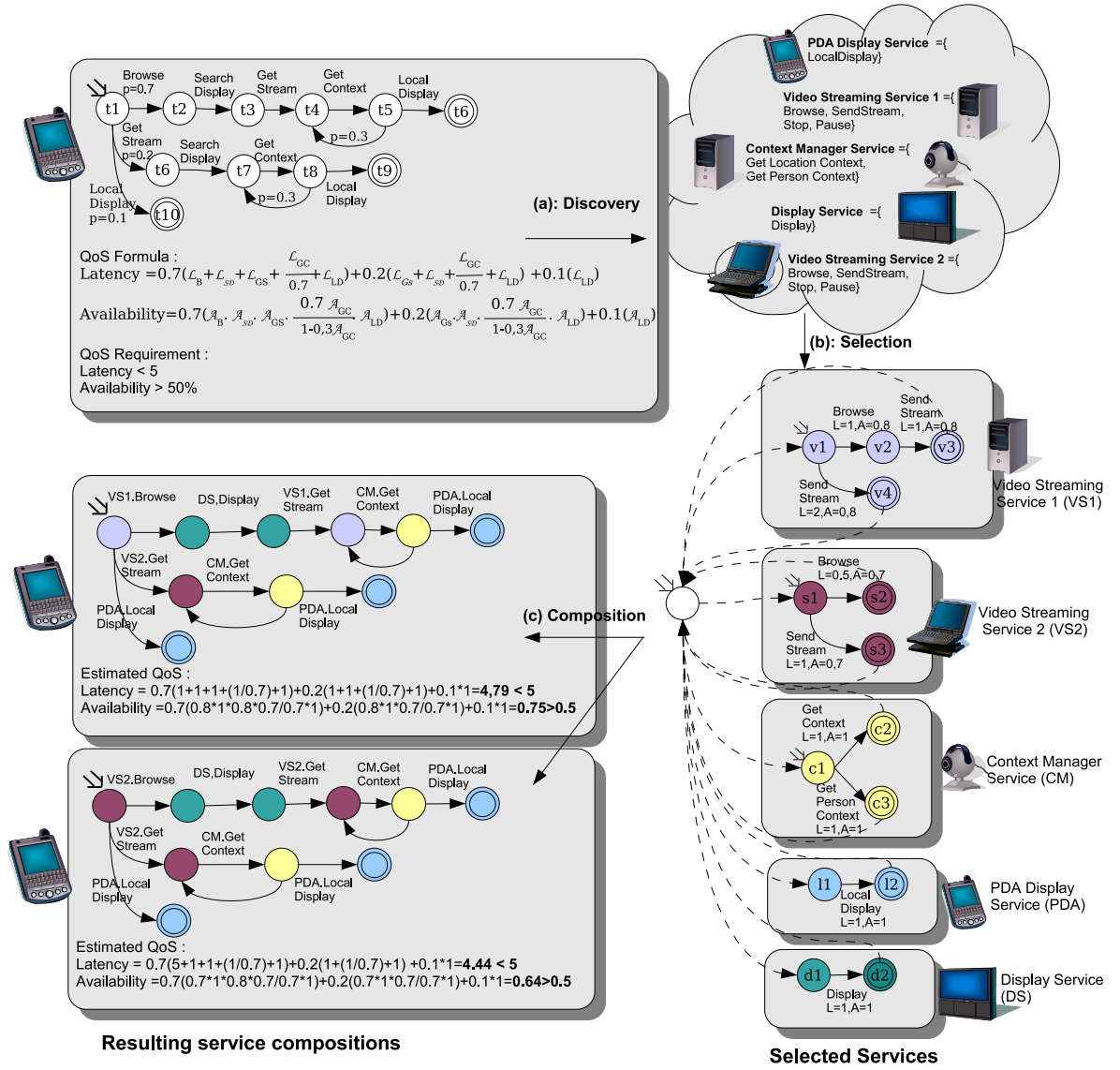
Fig. 10. Conversation Integration
