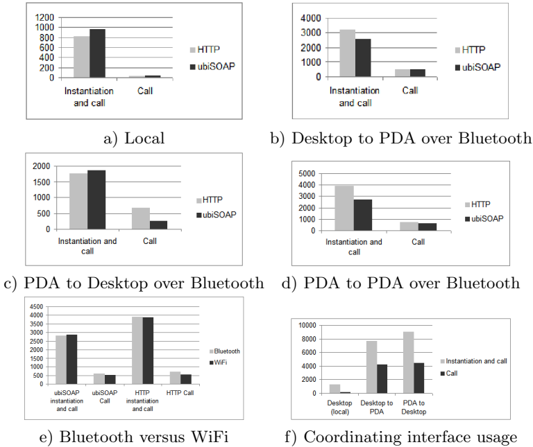
Fig. 5. ubiSOAP performance
