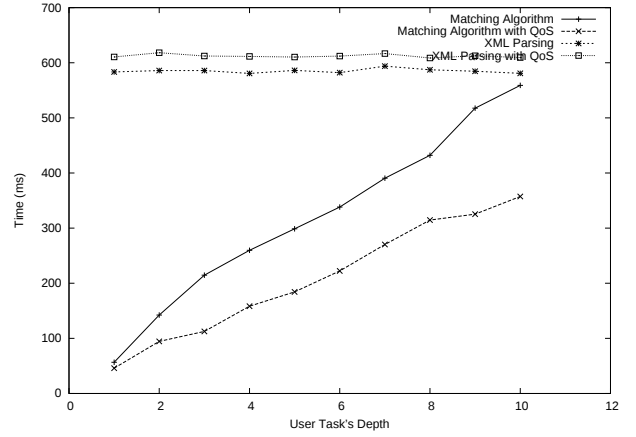
Figure 2: Performance of the Process Integration Algorithm with and without QoS
