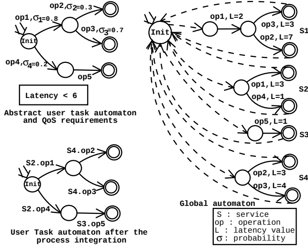
Figure 1: Example of the QoS-aware process integration
