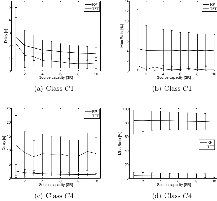
Figure 8: Diffusion delay and miss ratio (average value and its variance) as a function of the source upload capacity.
