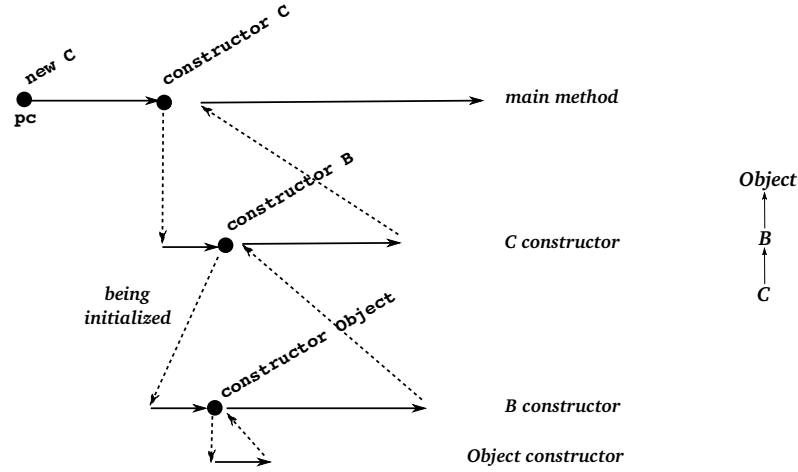
Figure 3.4: Object initialization process: example
