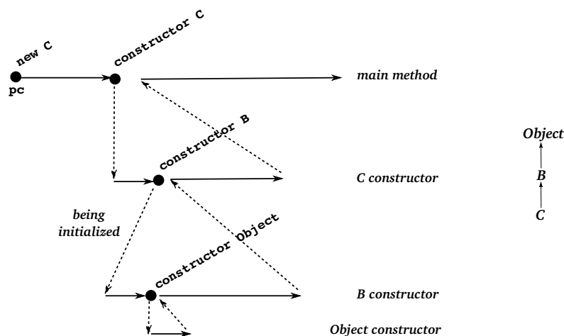
Figure 3.4: Object initialization process: example
